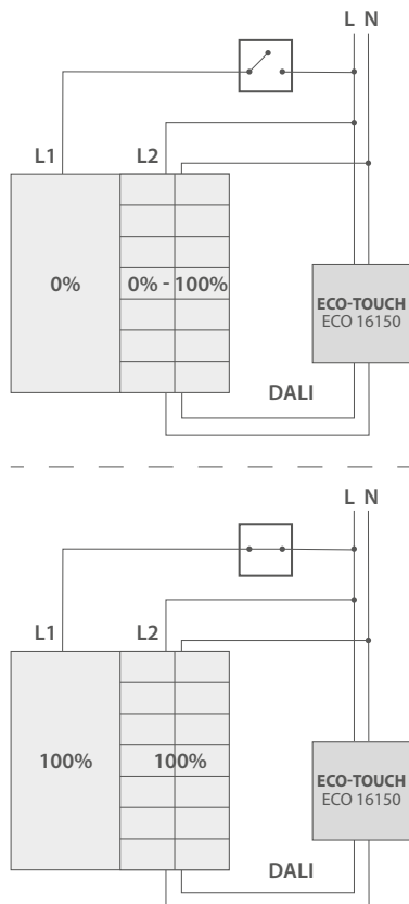
8a. SCHEMATIC WITH ECO 16150
