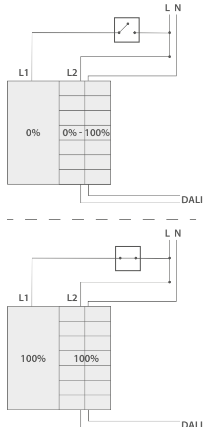
8b. SCHEMATIC
