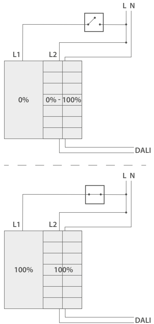
5b. SCHEMATIC
