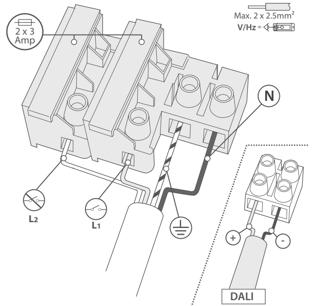
5b. SCHEMATIC
